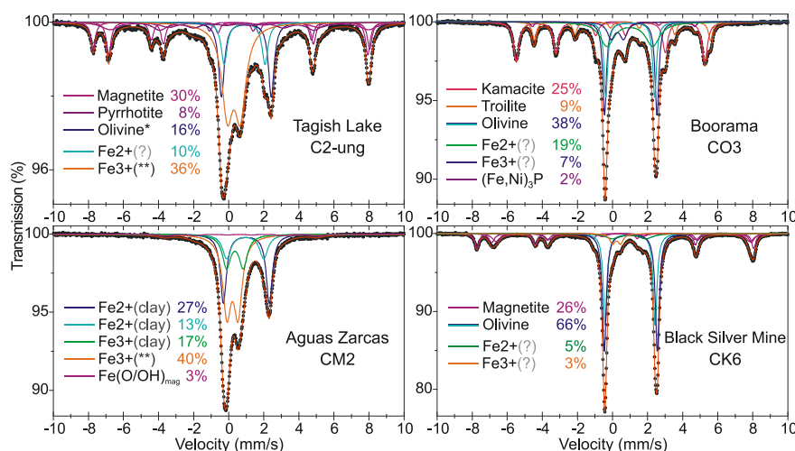
Figure 1. Mössbauer spectra of studied carbonaceous chondrites. Iron speciation, i.e. relative percentage distribution of Fe atoms into individual mineral phases and valence states is presented.
