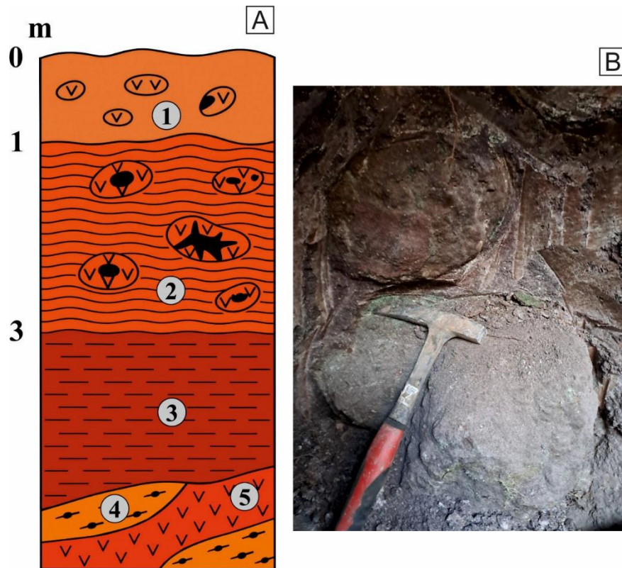
Figure 3. A. Geological profile of the agate-bearing zone near Nowy Kościół ("Piekielko" field): 1 - Weathered felsic volcanic rocks with agate-bearing lithophysae; 2 - Rhyolitic tuff with agate-bearing lithophysae; 3 - Rhyolitic tuff; 4 - Volcanic agglomerate; 5 – Rhyolite. (Lewczuk, as cited in Janeczek et al., 1991). B. Lithophysal agate in the weathered felsic volcanic rock. Photo: Piotr Sarul.
