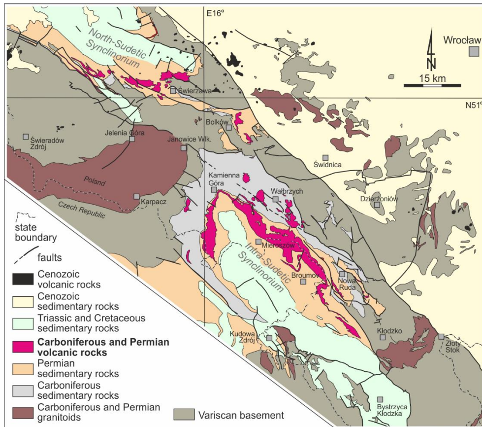
Figure 1. Geological map showing the North-Sudetic Synclinorium and Intra-Sudetic Synclinorium and the distribution of Carboniferous and Permian volcanic rocks in the Sudetes (modified from Kodym et al., 1967; Bossowski et al., 1981; Sawicki, 1988; Milewicz et al., 1989).
