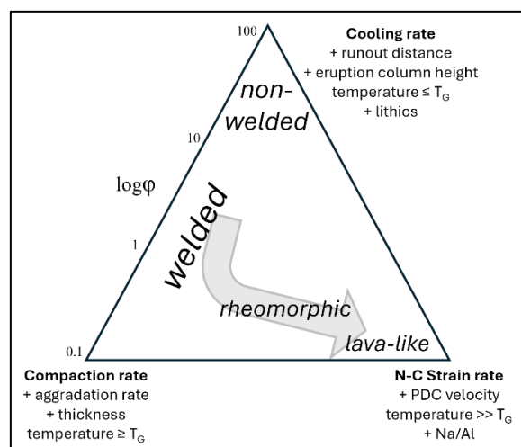
Figure 1. Controls on welding intensity in tuffs.
