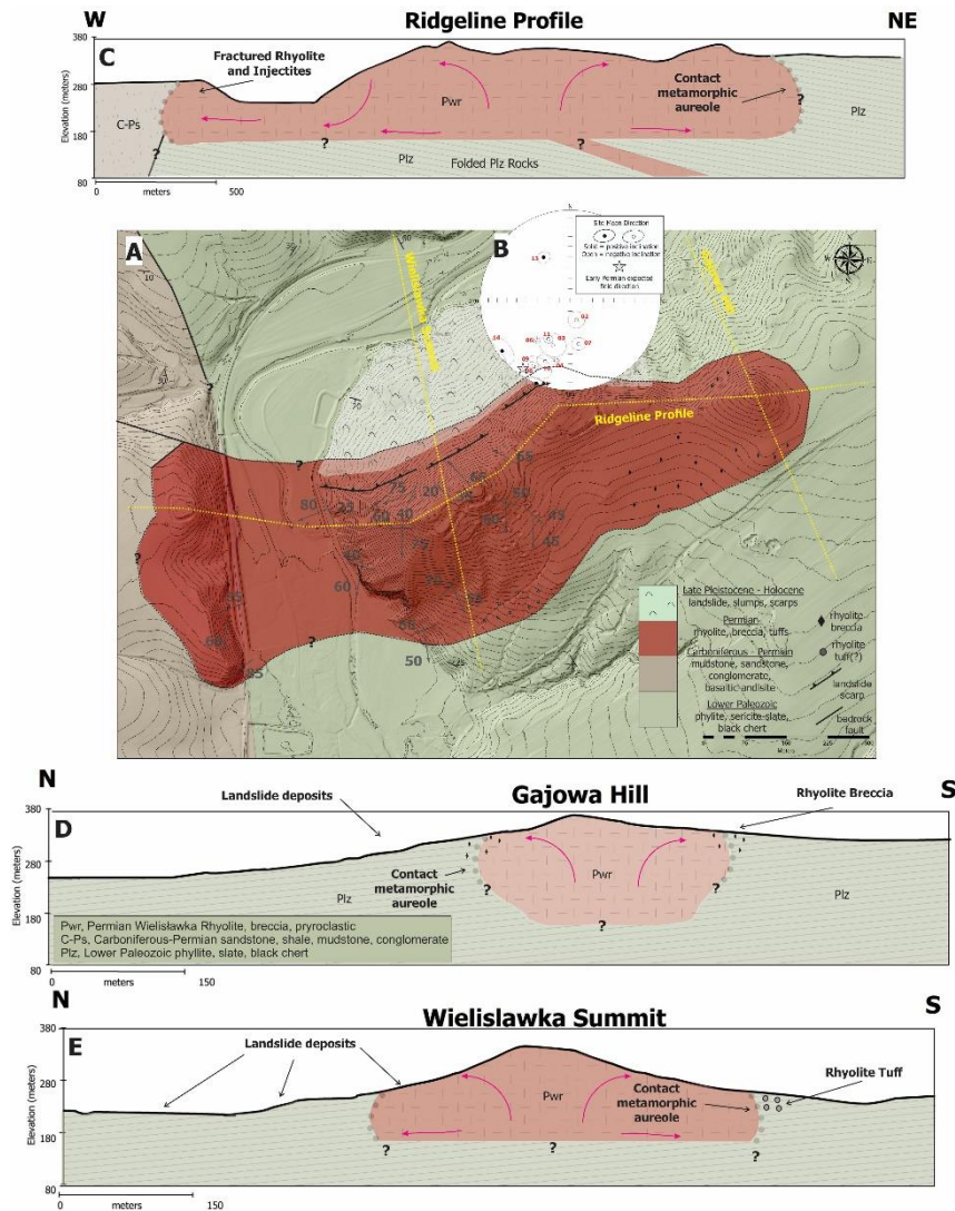
Figure 1. Bedrock geologic map (modified from Zimmermann & Kühn, 1918; Frąckiewicz, 1958; Milewicz & Kozdrój, 1995), paleomagnetic directions, anisotropy of magnetic susceptibility (AMS), and inferred magma flow of the Wielisławka Rhyolite. A) Geologic map of the Wielisławka Rhyolite showing the strike and dip of the macroscopic flow foliation and the trend and plunge of columnar joints. Yellow dotted lines indicate the location line of sections C-E. B) Lower hemisphere equal-area projection of the paleomagnetic site mean results. Star indicates the expected Permian field direction. C-E) Topographic profiles with idealized geologic interpretation of the subsurface and the inferred magma flow directions (magenta arrows). C) The cross-section line of section follows the ridgeline trail atop Wielisławka hill. The location of the magma ascent conduit is speculative; possible ascent pathways include a central pipe-like vent, a fissure vent parallel to the rhyolite outcrop, or a pre-existing fault or fracture zone. D) Line of section crossing Gajowa hill at the eastern part of the exposed rhyolite. E) Line of section crossing Wielisławka summit. Explanation: Pwr, Permian Wielisławka Rhyolite, breccia, pyroclastic C-Ps, Carboniferous-Permian sandstone, shale, mudstone, conglomerate; Plz, Lower Paleozoic phyllite, slate, black chert.
