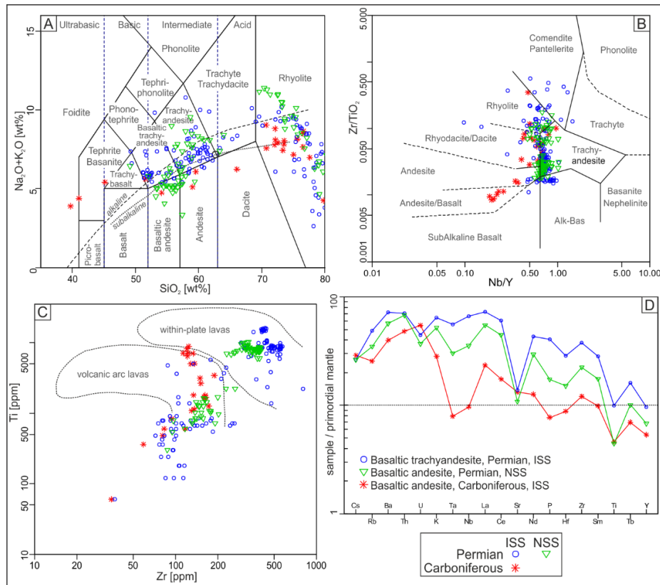
Figure 2. Selected diagram illustrating the classification and geochemical characteristics of the Carboniferous and Permian volcanic rocks of the Sudetes (237 samples; ISS – Intra-Sudetic Synclinorium, NSS – North-Sudetic Synclinorium; data from Awdankiewicz, 1998, 1999, 2006; Szczepara, 2018, and unpublished results). A. The total alkalis – silica (TAS) diagram (after Le Maitre et al., 2002). The boundaries of the alkaline and subalkaline series after Irvine & Baraggar (1971; dashed line) and after Kuno (1966; dotted line). B. The \text{Zr}/\text{TiO}_2 -Nb/Y diagram (Winchester & Floyd, 1977). C. Ti-Zr discrimination plot (Pearce, 1983). D. Primordial mantle-normalized plots of least evolved samples from the main volcanic suites (normalization after Wood et al., 1979).
