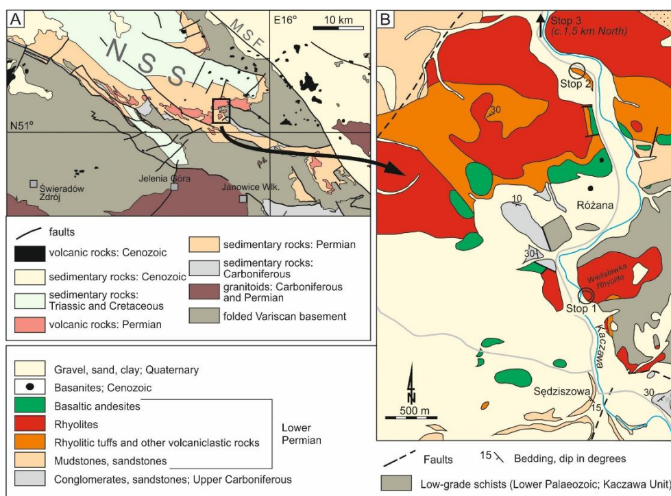
Figure 1. A. Geological sketch map of the North-Sudetic Synclinorium (NSS; modified from Bossowski et al., 1981; Milewicz et al., 1989) showing the field trip area (rectangle near the centre). MSF - Marginal Sudetic Fault. B. Geological map of the field trip area (modified from Frąckiewicz, 1958; Milewicz & Kozdrój, 1995) with location of the field stops 1-3.
