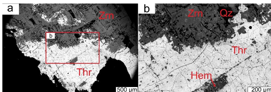
Figure 1. BSE images of sample 2-8-6: a) thorite (Thr) in contact with porous zircon (Zrn); b) enlarged view of irregular zircon domains penetrating thorite along the fractures. Qz - quartz, Hem - hematite.
